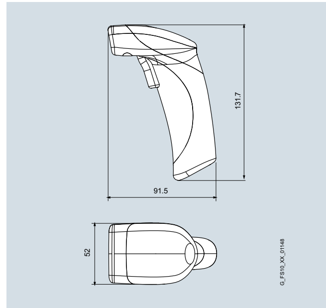
SIMATIC MV320 optical handheld reading device
