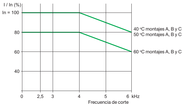
ATV 61HD90Y (1)
