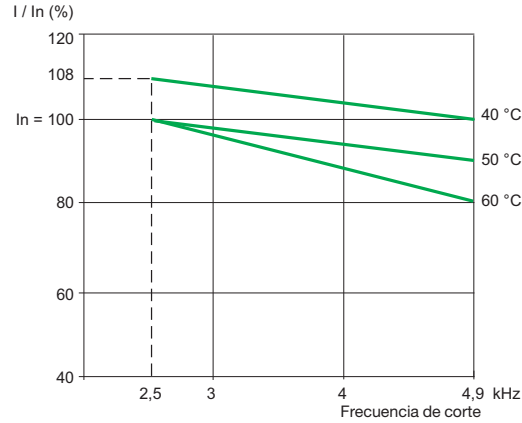
ATV 61HC13Y
