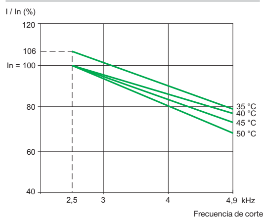
ATV 61EXS5C25N, ATV 61EXS5C31Y
