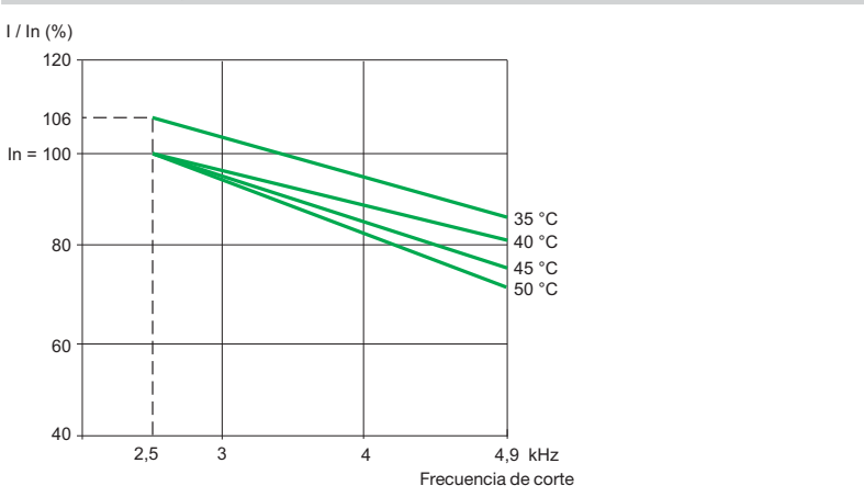
ATV 61EXS5C13N, ATV 61EXS5C16Y
